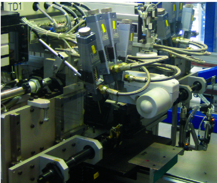
DOPAG dispensing valves automatically dispensing grease onto the linear actuators
